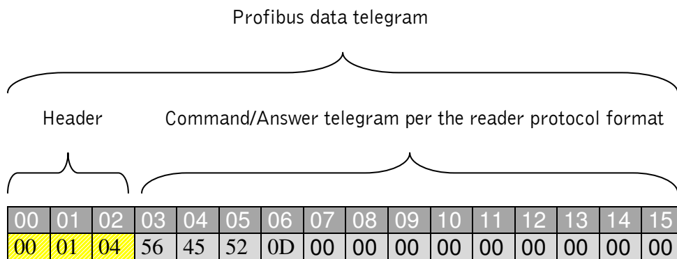
Figure 2-1 Character sequence of the profibus data telegram
